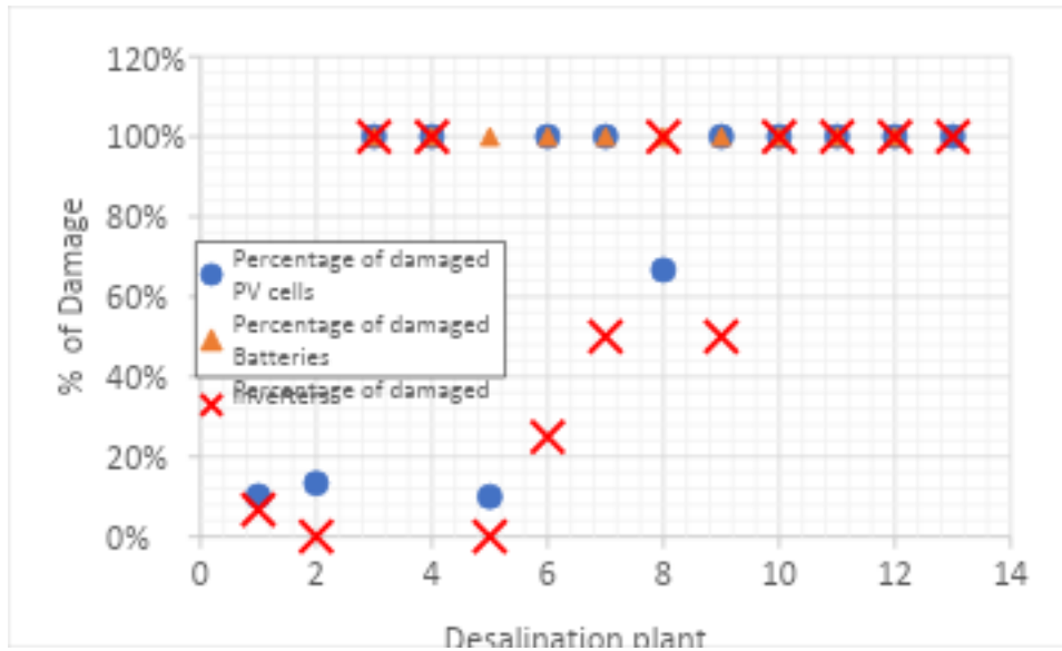
Figure 11, % of damage in solar systems main components
